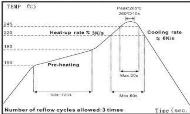
IR Reflow Soldering
