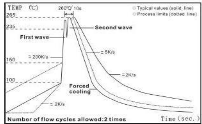
Wave Soldering (Flow Soldering)
