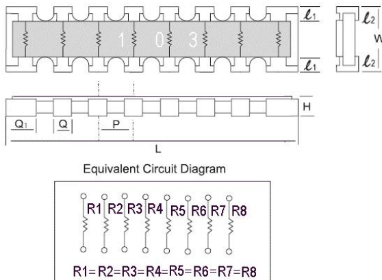
0402&0603 16P8R D Type
