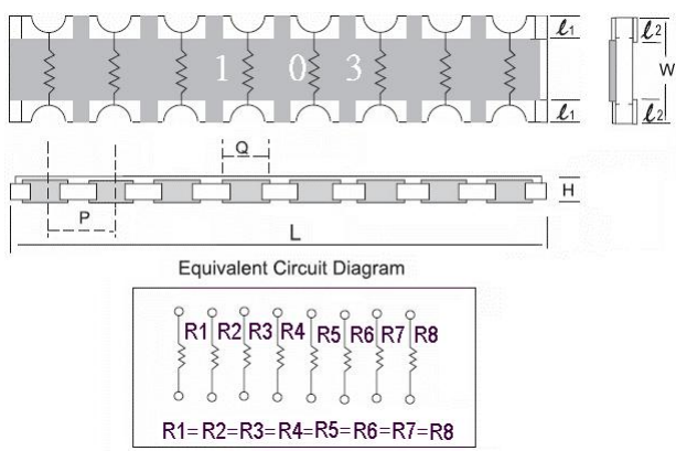
0402&0603 16P8R C Type
